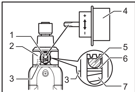
► 1. Adjust ring 2. Ring 3. Scale 4. Adjust grip 5. Hole for adjust grip 6. Yellow line 7. Compression spring
